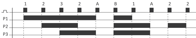
Group system diagram
